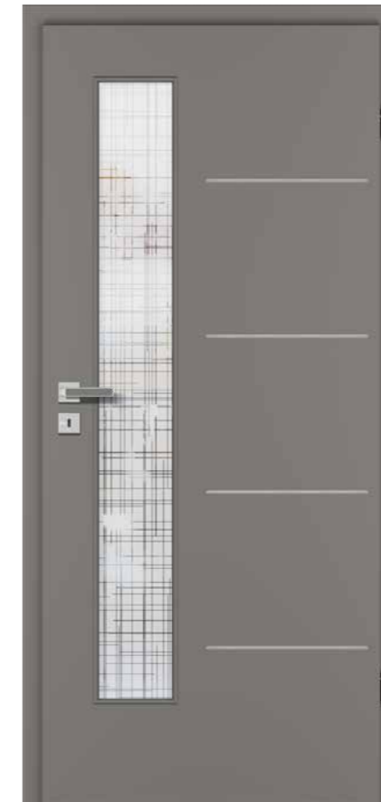
2 MODELL: AURA A834-LA4S, G-TEC® STAUBGRAU GLAS: PANNO, Design-Ornamentglas BESCHLAG: QUADRAL-Inlay, Flach-Rosette, mit Schlüssel-Rosette MODEL: AURA A834-LA4S, G-TEC® DUSTY GREY GLASS: PANNO, Patterned design glass FITTING: QUADRAL-Inlay, Flat rosette, with keyhole rosette
